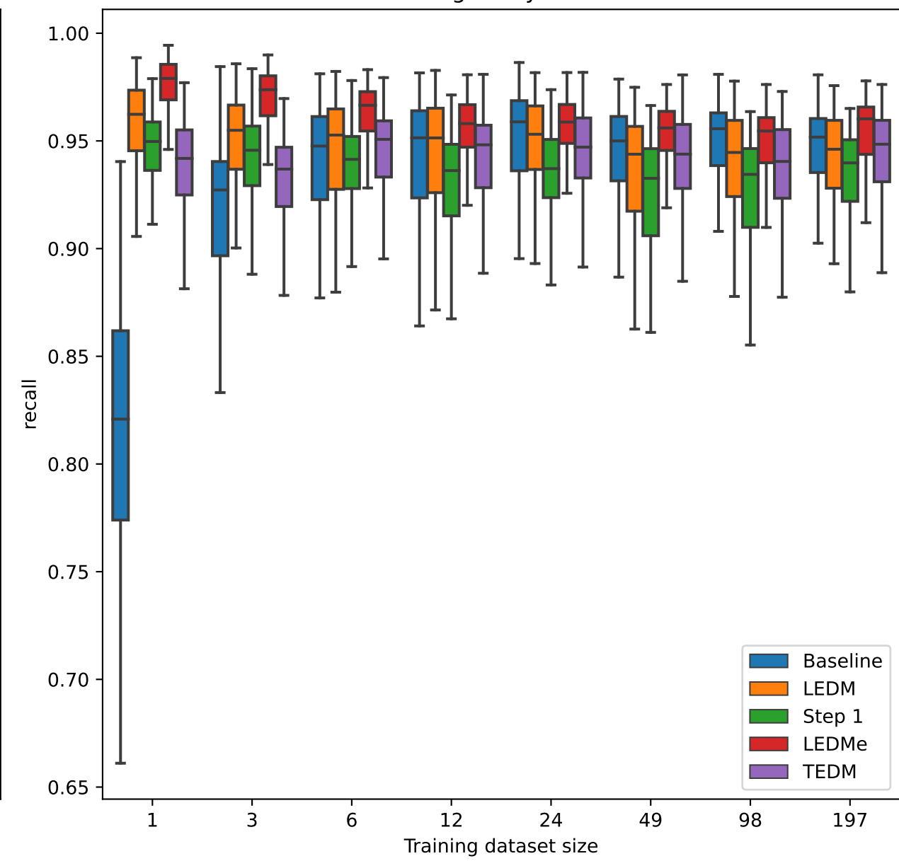
Montgomery recall
