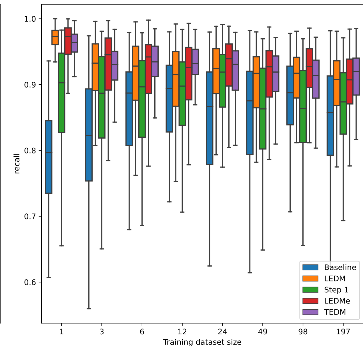
Montgomery recall
