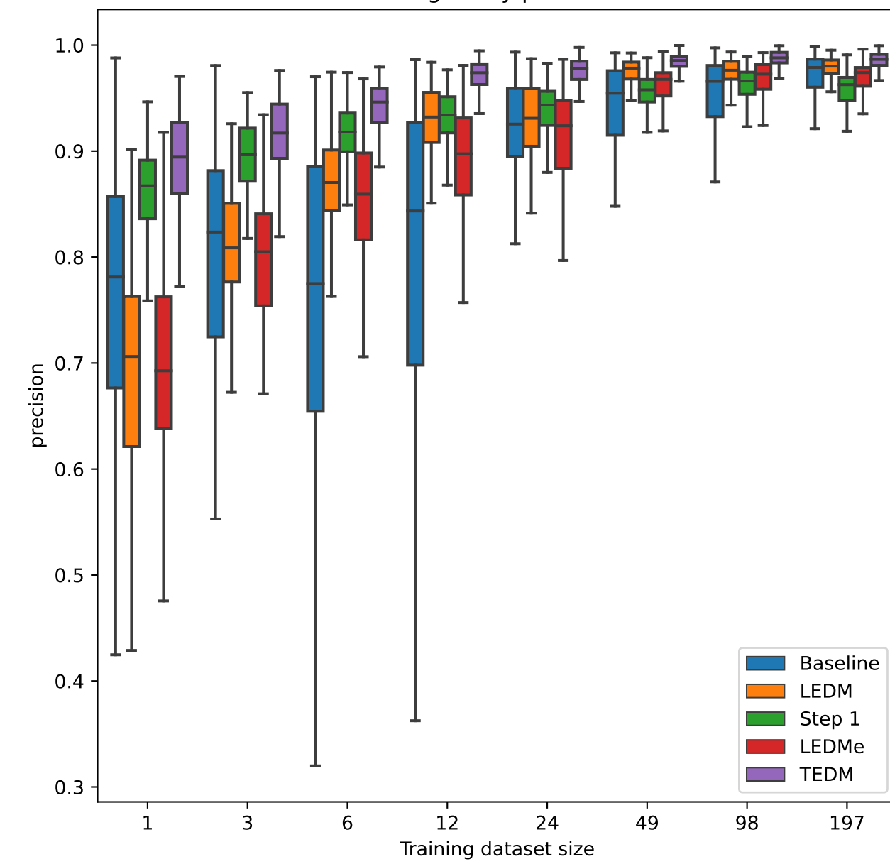
Montgomery precision
