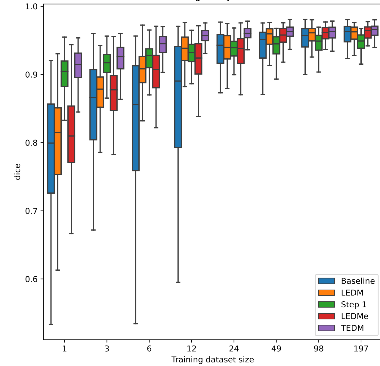
Montgomery dice
