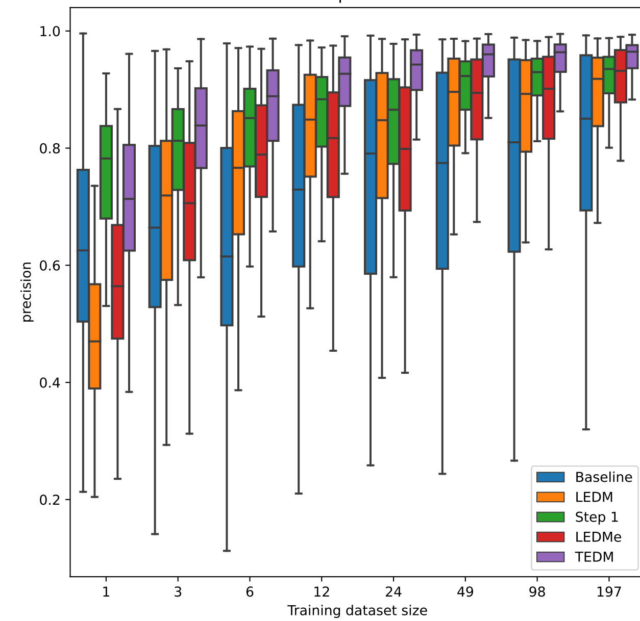
Montgomery precision
