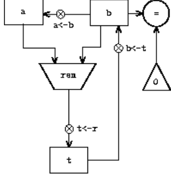
Figure 5.1: Data paths for a GCD machine.
