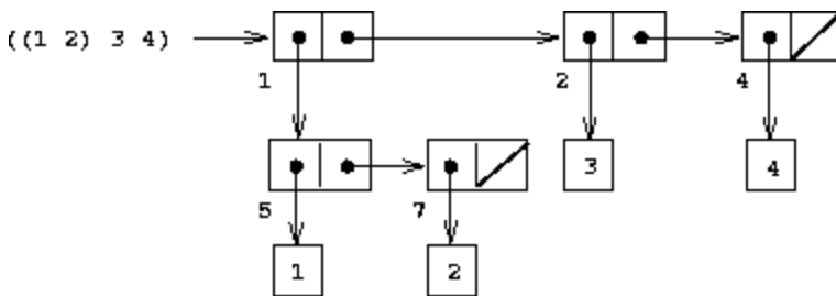
Figure 5.14: Box-and-pointer and memory-vector representations of the list ((1\ 2)\ 3\ 4) .
