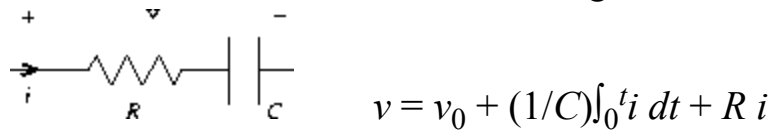
Figure 3.33: An RC circuit and the associated signal-flow diagram.
