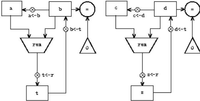
Figure 5.7: Portions of the data paths and controller sequence for a machine with two GCD computations.
