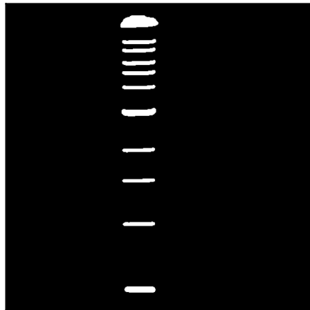
Mask Prediction
