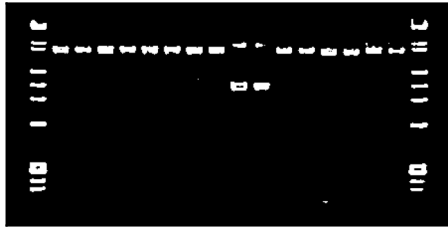
Mask Prediction
