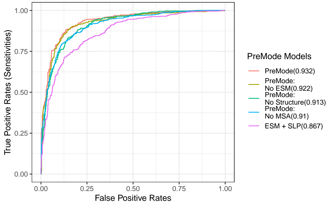
ROC curve on pathogenicity task
