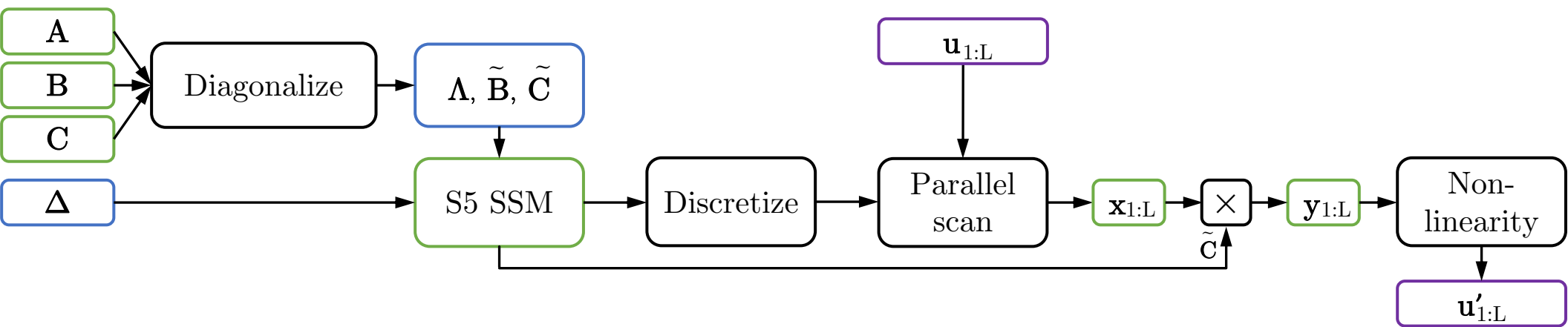
Learnable parameter Operation Instantiated variable Message between layers
