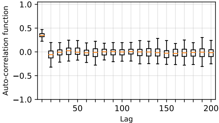
Importance sub-sampling with preconditioning
