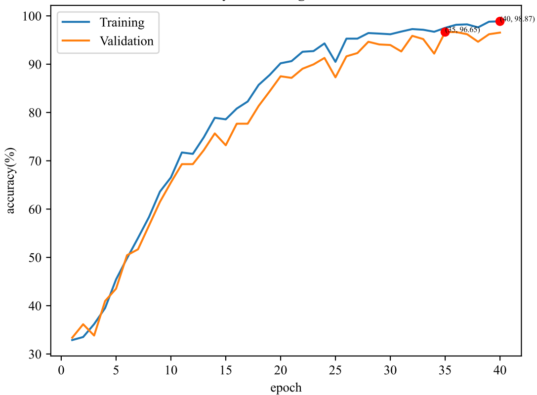
Accuracy of training and validation
