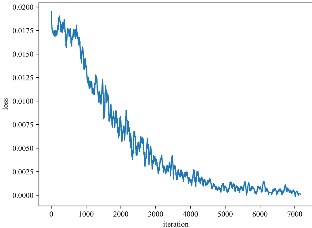
Loss curve
