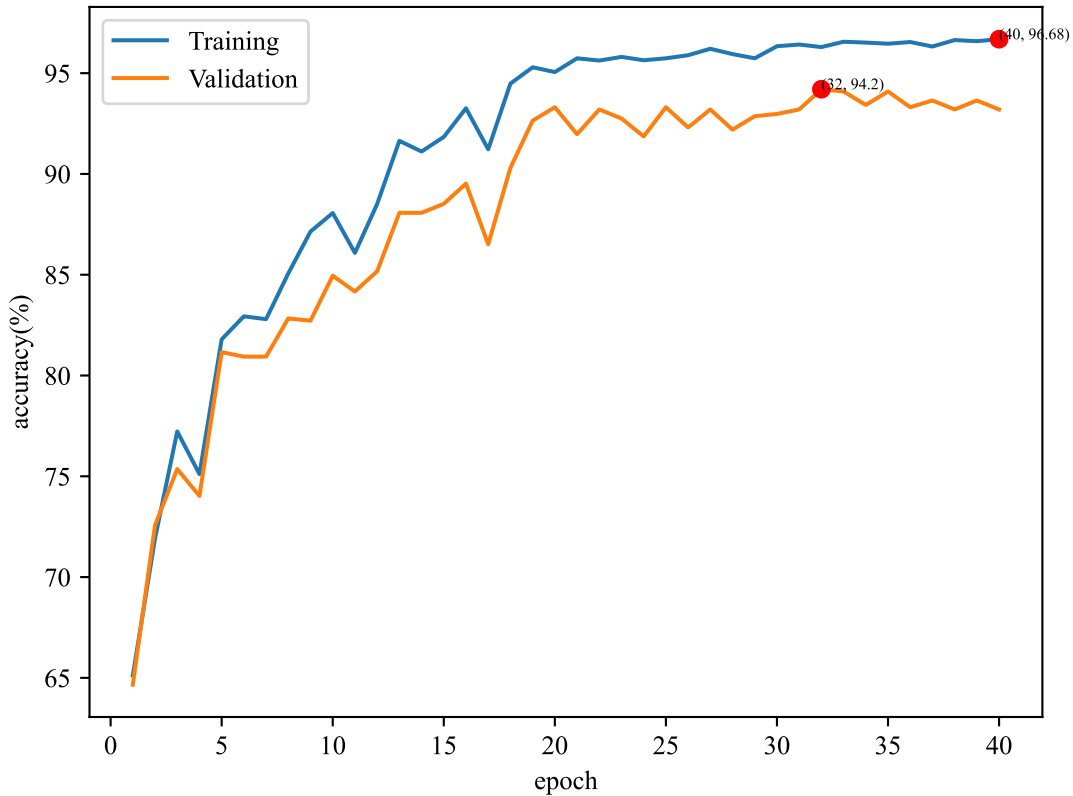
Accuracy of training and validation
