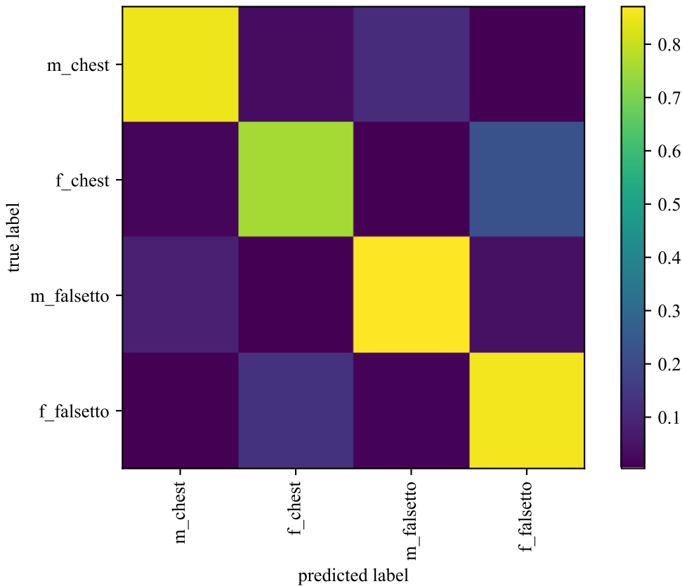
Confusion matrix
