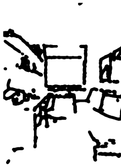
Scribbles (synthesized)
